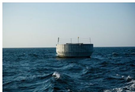
Fig. 8: Offshore anchored concrete foundation
