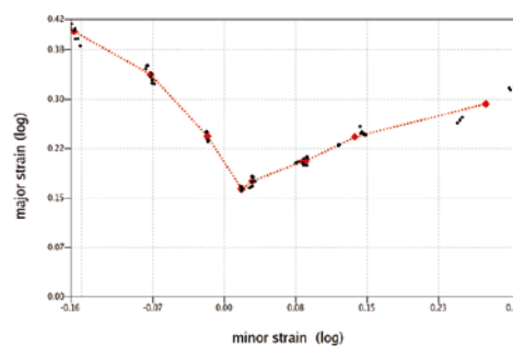
Fig. 9: FLC of a 1 mm thick steel sheet metal
