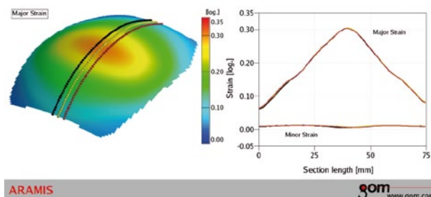
Fig. 8: Sections with respective section data. The diagram shows the major and the minor strain over the section length
