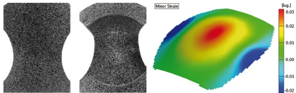
Fig. 3: Undeformed and deformed Nakajima specimens with stochastic pattern
