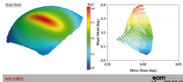
Fig. 7: Deformation of the sheet metal specimen with the current major strain (color representation, measured by ALCAN)
